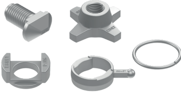
KONTEYNER KİLİDİ İÇ TAKIM 52 MM CONTAINER LOCK INNER TOOL 52 MM
